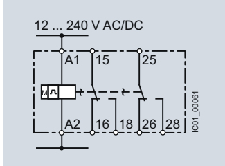
7PV1508-1BW30 Flashing, starting with interval
