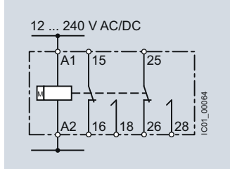
7PV1508-1BW30 Passing make contact
