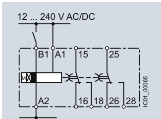
7PV1508-1BW30 ON and OFF-delay
