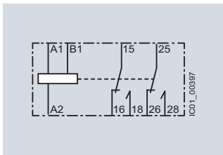
3RP2505-.B (L) Pulse-delayed with control signal (fixed pulse (at 1 s) and settable pulse delay)
