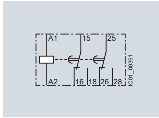
3RP2505-.B (A) ON-delay
