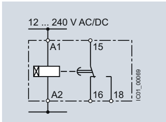
7PV1518-1AW30 ON-delay
