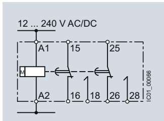
7PV1508-1BW30 Fixed pulse after ON-delay
