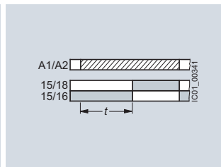
K Pulse-delayed (fixed pulse (at 1 s) and settable pulse delay)
