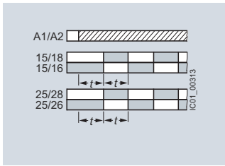
D Flashing, symmetrical, starting with interval
