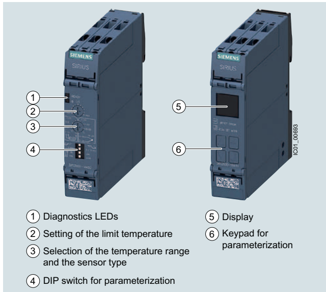
SIRIUS 3RS25 analog multi-function device
