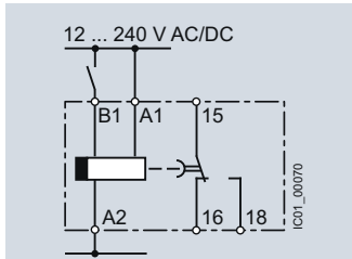
7PV1538-1AW30 OFF-delay with control signal
