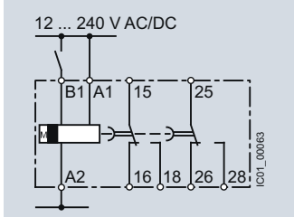
7PV1508-1BW30 OFF-delay with control signal
