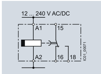
7PV1540-1AW30 OFF-delay without control signal
