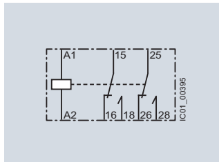
3RP2505-.B (E) Passing make contact, interval relay
