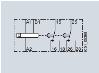
3RP2505-.B (H) Additive ON-delay, instantaneous OFF with control signal
